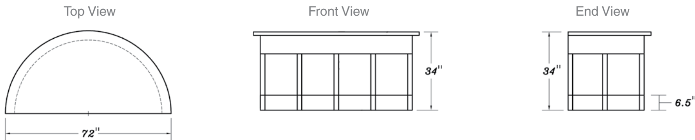
Display Table with Open Area – CTDT-200
