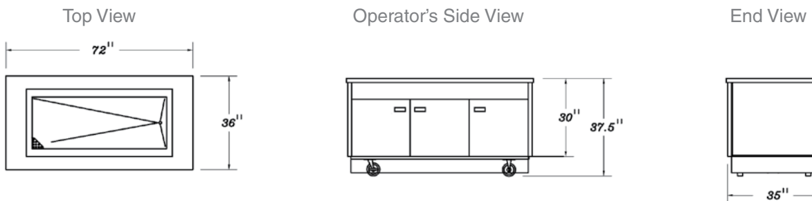
Display Table with Cold Pan – CTDT-300
