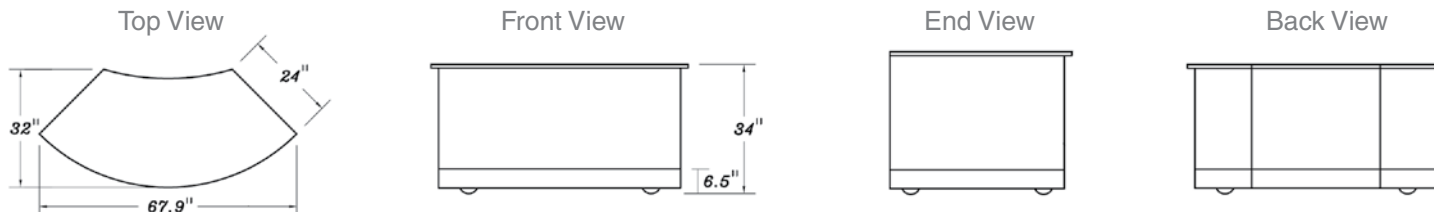
Display Table with Storage – CTDT-100
